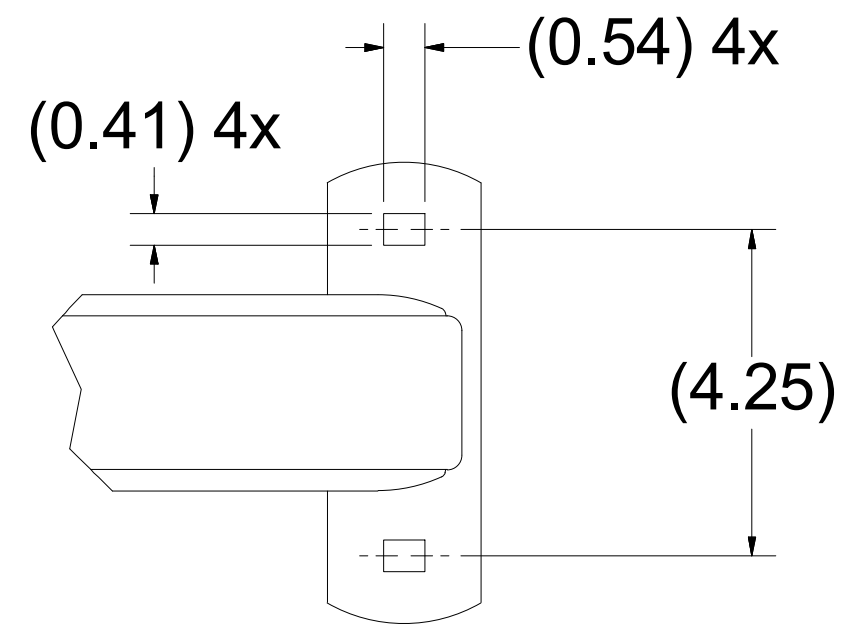
FOOT DETAIL A
