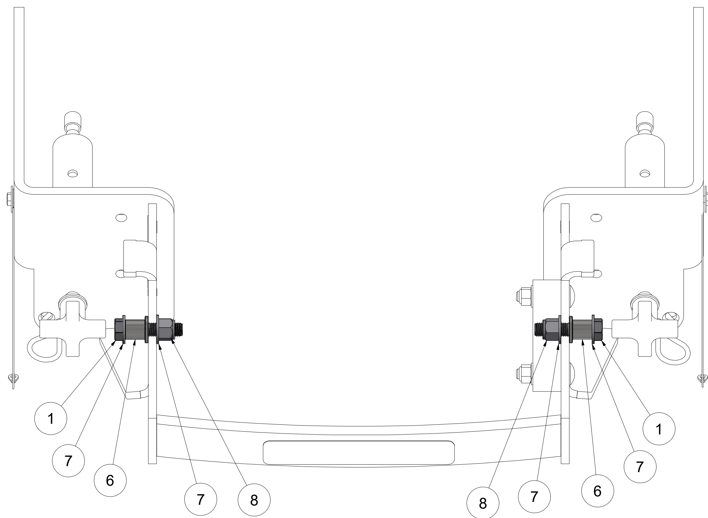
APEX 2 PIVOT BOLT STACK
