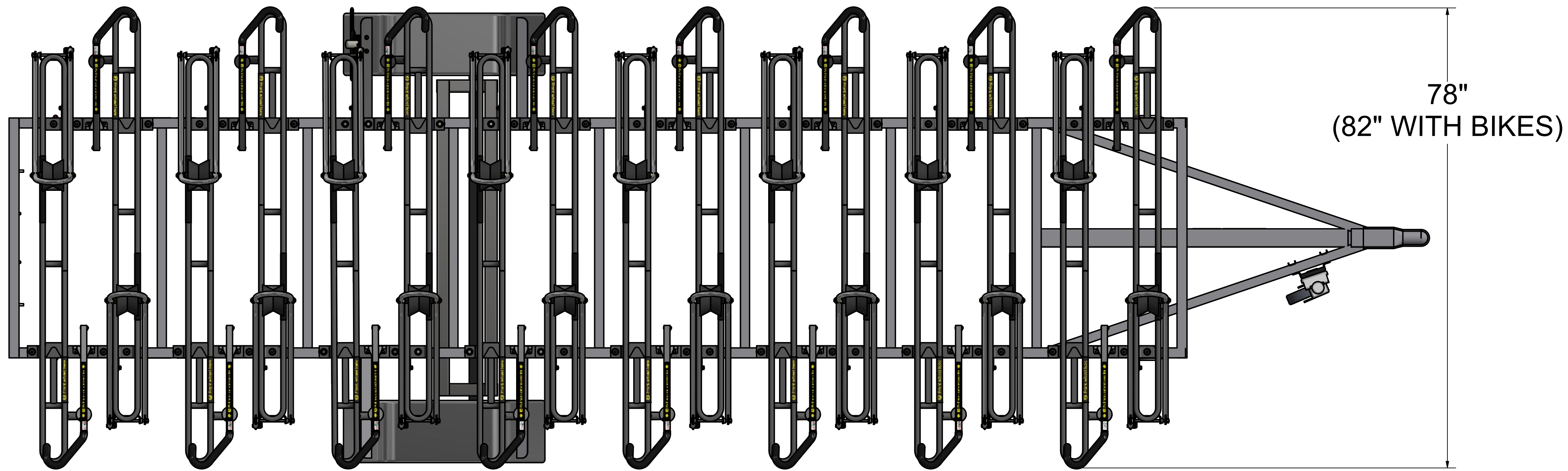
16 BIKE TRAILER, 234" (240" WITH BIKES) 12 BIKE TRAILER, 186" (192" WITH BIKES)
