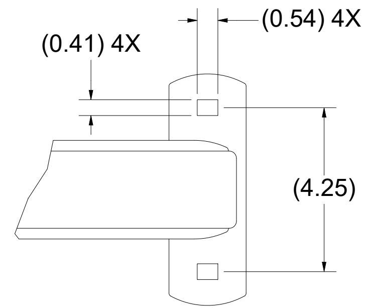
FOOT DETAIL A
