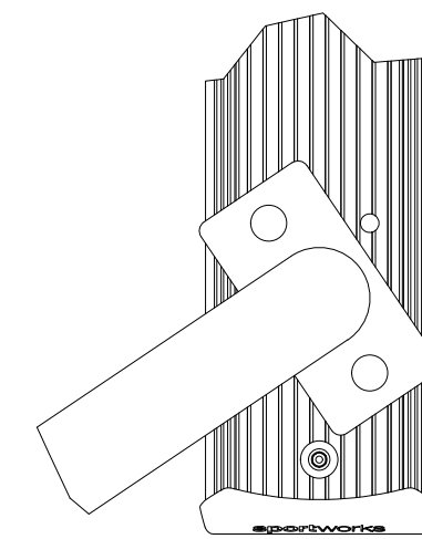
DETAIL WITH STANDARD RACK FOOT
