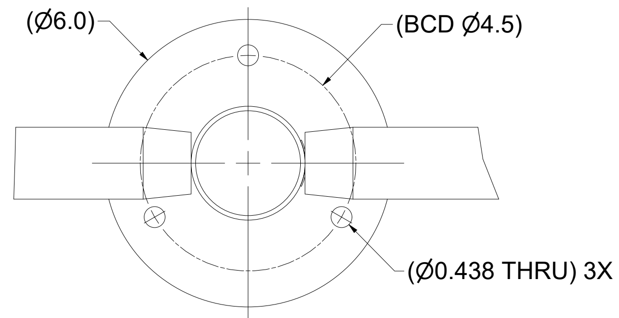
FOOT DETAIL A
