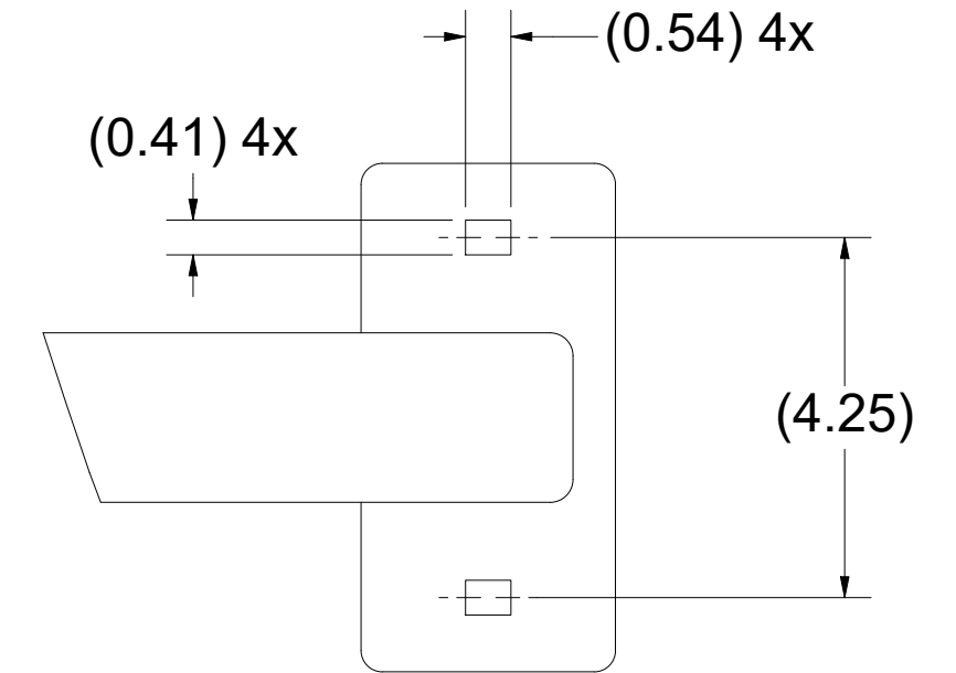
FOOT DETAIL A
