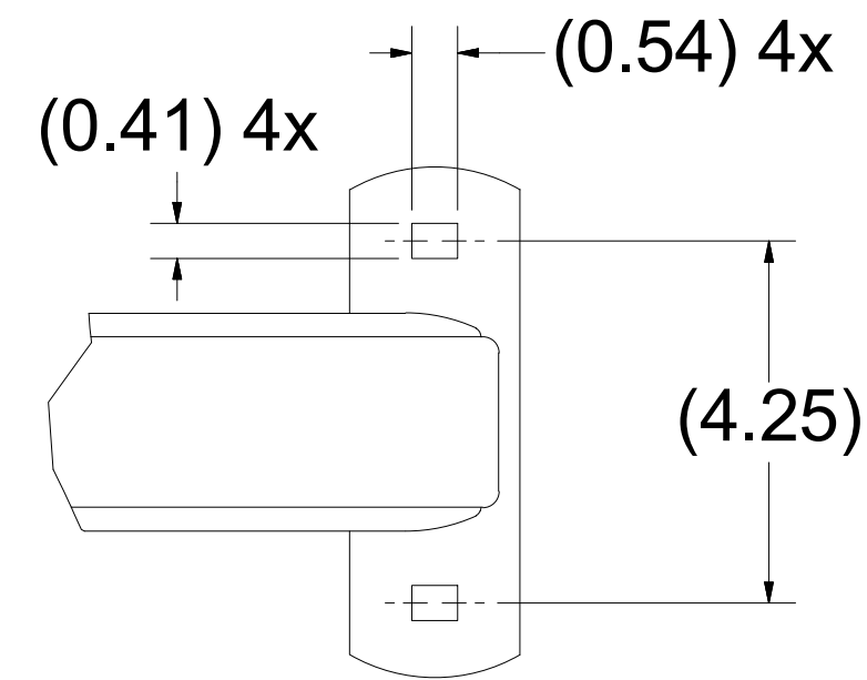
FOOT DETAIL A
